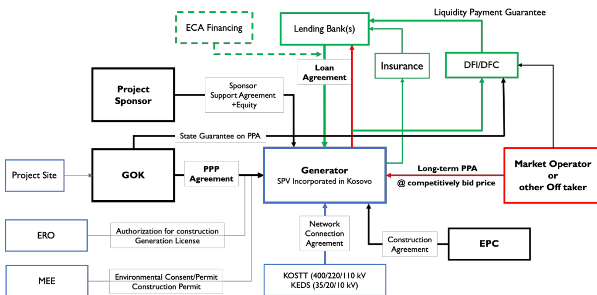
Figure 2: Structure of a 50 MW Solar PV Project
