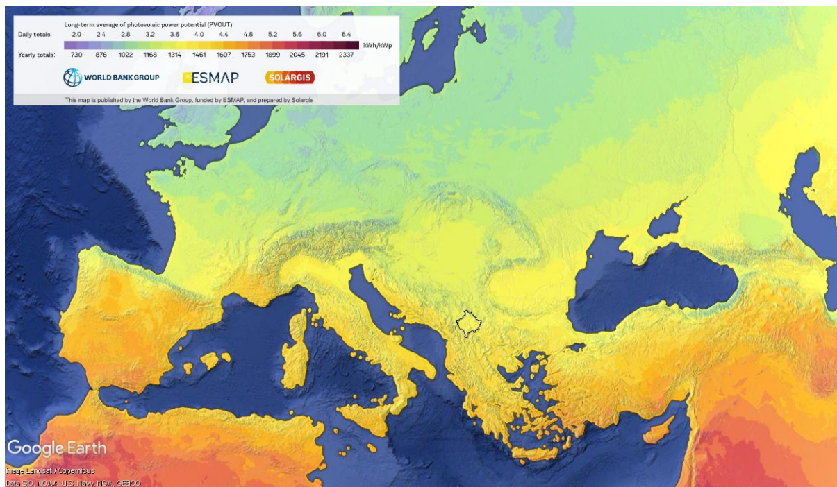
Figure 1 Long-term average photovoltaic power potential (PVOUT)
