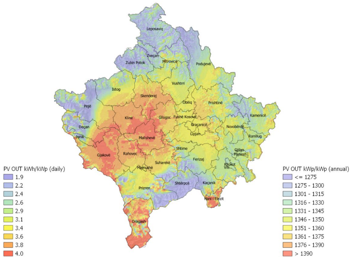
Figure 2 PV power output (PVOUT) in Kosovo.
