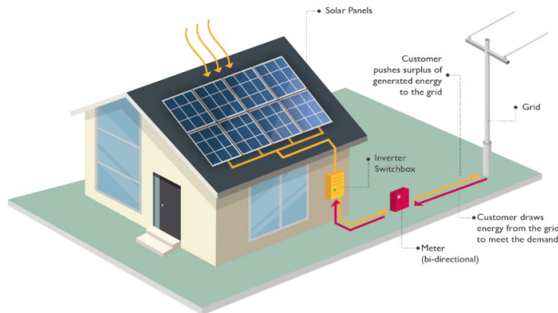
Figure 6 Household with a status of a Prosumer and solar PV installation
