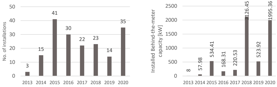
Figure 29 Number and capacity of Behind-the-meter installations 2013 - 2020
