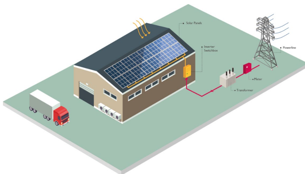
Figure 7 Business customer with Behind-the-meter solar PV installation
