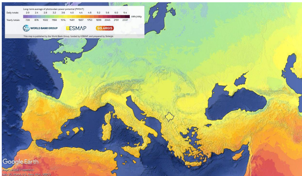
Figure 1 Long-term average photovoltaic power potential (PVOUT).
