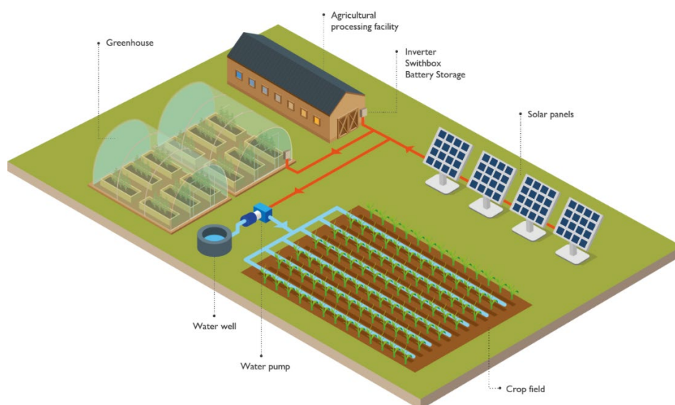
Figure 7 Off-grid solar PV generator in agriculture
